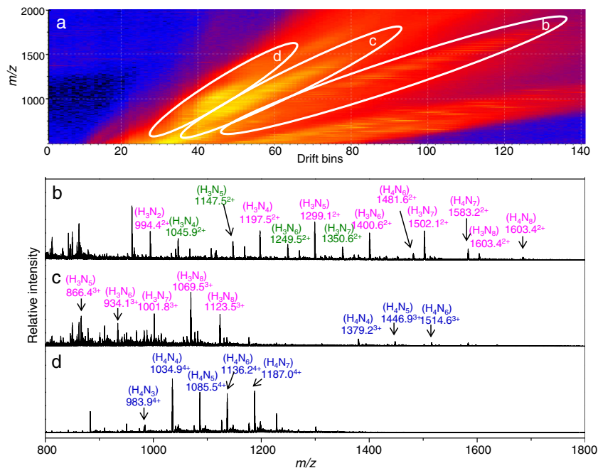
Figure 3. (a) IMS-MS ( m/z versus drift bins) distribution of the ovomucoid glycopeptides from the C18 fraction f7. The white ovals designate the extracted ion bands shown in the corresponding panels below (b)–(d). Glycopeptides are labeled in color (green: FPN*ATDK; pink: SIEFGTN*ISK; blue: TYGNKCNFCNAVVESN*GTLTLSHF; the * symbol indicates the glycosylation site), and the associated glycan forms are shown in the parentheses above the m/z labels. The charge state of each ion is labeled in superscript to the m/z label
