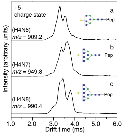
Figure 5. IMS distributions of the quintuply charged glycopeptide series containing the peptide TYGN KCNFCNAVVESN*GTLTLSHF modified by various glycans H_4N_x ( x = 6-8 ) shown in each panel. Glycans are shown in cartoon representations: blue square-GlcNAc; green circle-mannose; yellow circle-galactose; the big parentheses are used to indicate the possible positions where the terminal galactose can be attached. The glycan structures are from References [41] and [75]
