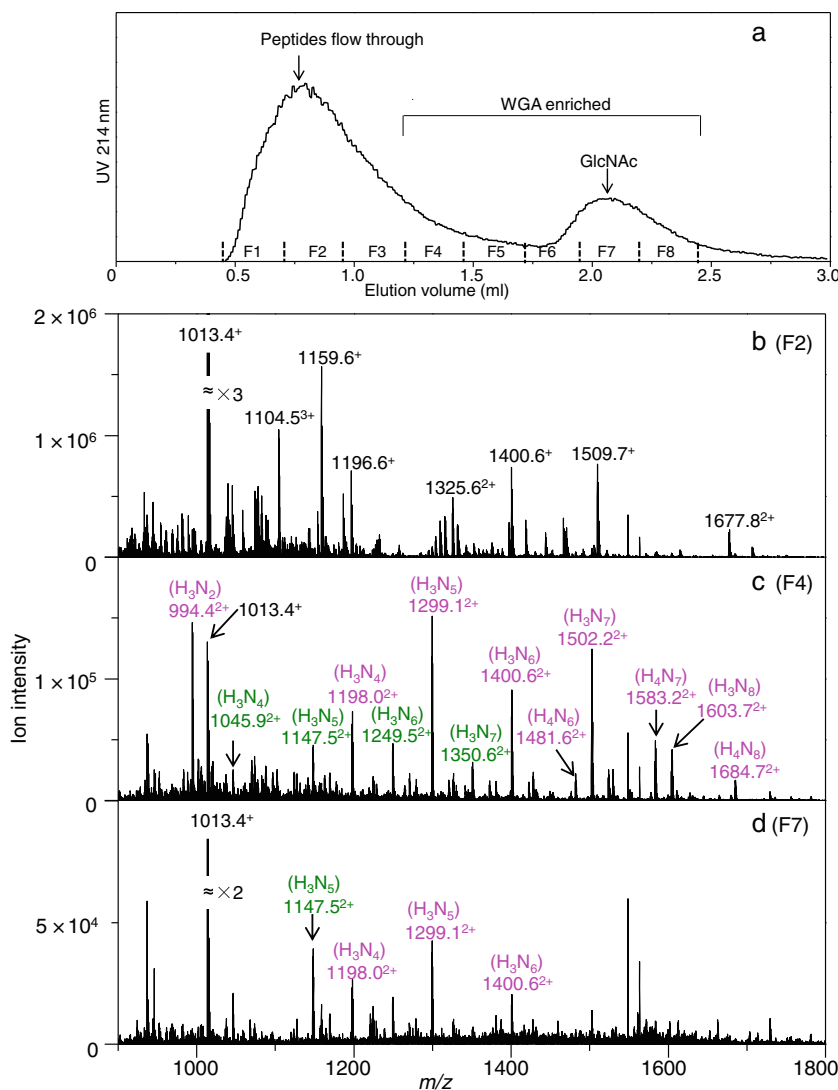
Figure 1. (a) UV absorption trace at 214 nm of the lectin affinity chromatography (LAC) enrichment of the ovomucoid digest using an isocratic buffer condition. Vertical lines immediately above the X axis indicate positions of the fractions collected (F1–F8). The Orbitrap MS analysis of species in fractions F2, F4, and F7 are displayed in panels (b), (c), and (d), respectively. Each spectrum was obtained by integrating the elution window corresponding to all peptides. Glycopeptides are labeled in color (pink: SIEFGTN*ISK; green: FPN*ATDK. The * symbol indicates the glycosylation site), and the associated glycan forms are shown in the parentheses above the m/z labels. Non-glycosylated peptides are indicated by black m/z labels. Charge state of each ion is labeled in superscript to the m/z label
