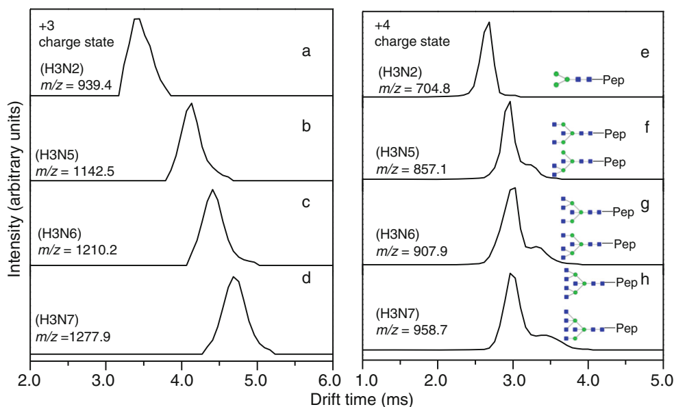
Figure 4. IMS distributions of the triply charged [panels (a)–(d)] and quadruply charged [panels (e)–(h)] glycopeptides containing the peptide GAEVDCSRFPN*ATDKEGK modified by various glycans H_3N_x ( x = 2, 5-7 ) shown in each panel. The glycan structures are drawn in cartoon representations: blue square–GlcNAc; green circle–mannose. The glycan structures are from Reference [41]
