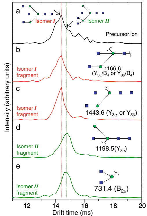
Figure 6. (a) IMS distribution of the precursor glycan ion [H_3N_5 + 2Na]^{2+} ( m/z = 964.8 ). Two isomeric structures, isomer I and isomer II , are shown in cartoon representations as described in Figure 4. CID spectra of this precursor ion are taken across entire the drift time range. The extracted fragment ion drift time distributions (XFIDTD) of the unique fragments to isomer I (red traces) and isomer II (green traces) are shown in panels (b)–(e). Fragments at m/z = 1166.6 and 1443.6 are unique to isomer I . Fragments at m/z = 1198.5 and 731.4 are unique to isomer II . The fragments are singly sodiated. The dashed lines are drawn to guide the eye
