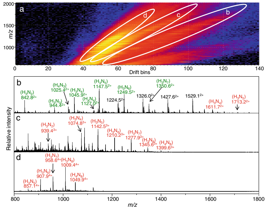
Figure 2. (a) IMS-MS ( m/z versus drift bins) distribution of the ovomucoid glycopeptides from the C18 fraction f5. The white ovals designate the extracted ion bands shown in the corresponding panels below (b)–(d). Glycopeptides are labeled in color (green: FPN*ATDK; red: GAEVDCSRFPN*ATDKK; the * symbol indicates the glycosylation site), and the associated glycan forms are shown in the parentheses above the m/z labels. The charge state of each ion is labeled in superscript to the m/z label
